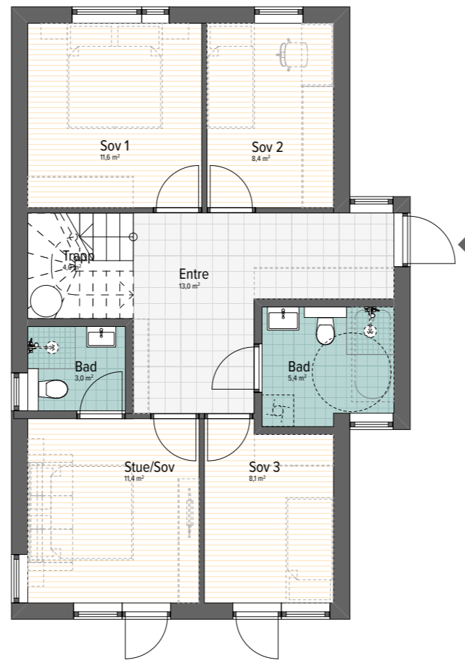
Plan 1. etasje BRA = P-rom 68,0 m 2
